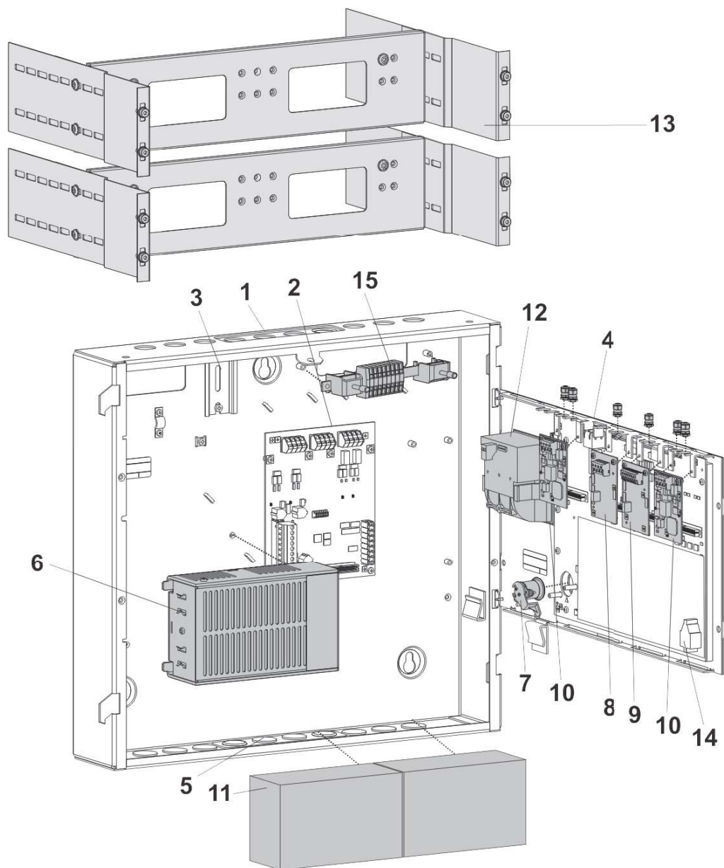
Fig. 5: Layout of FT724
