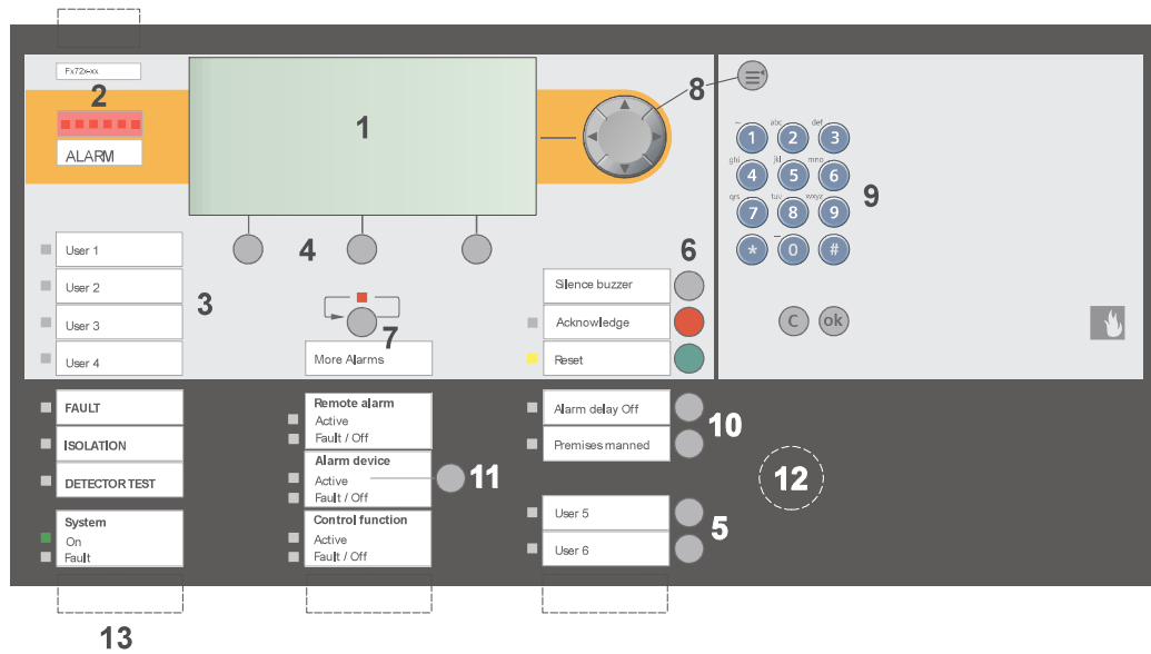
Fig. 4: Indication and operating elements
