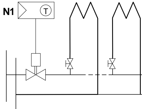
Room thermostat for a hydronic zone control system (radiator/floor heating)
