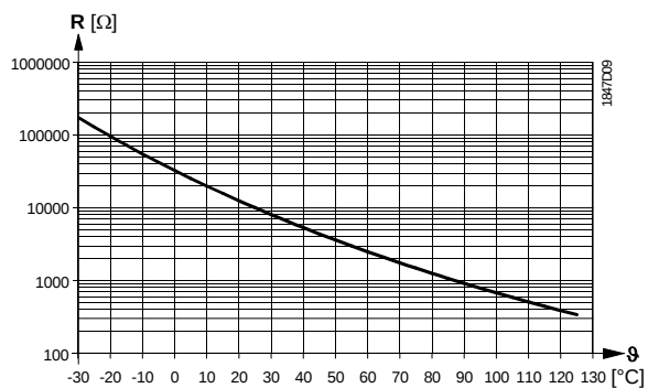
NTC 10k
